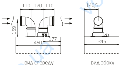
Nuvola Platinum+ / Nuvola Duo-tec+
