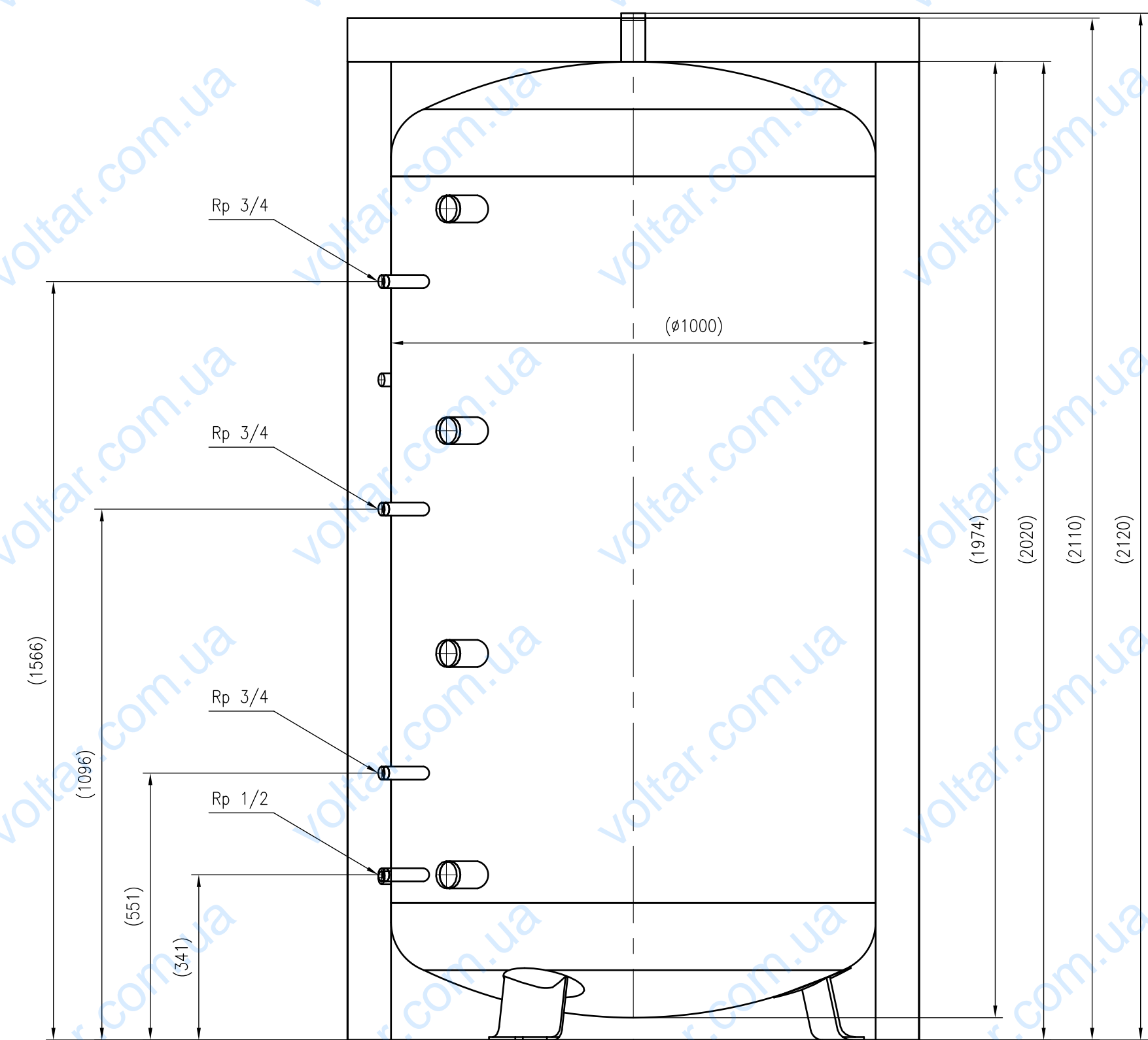
Side view
