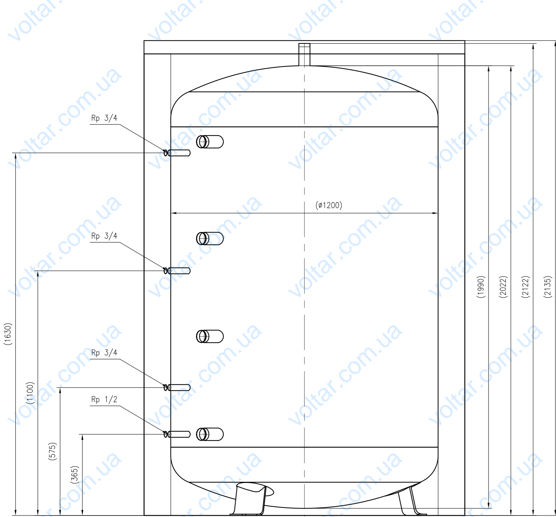
Side view
