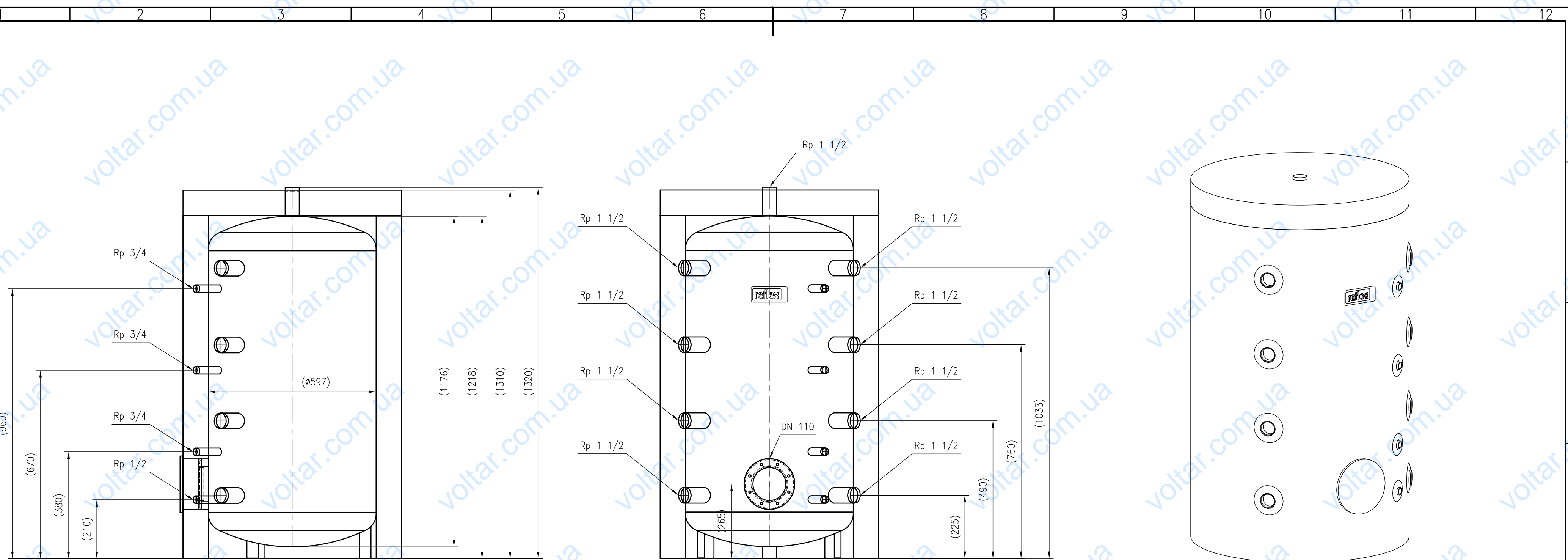
Side view
