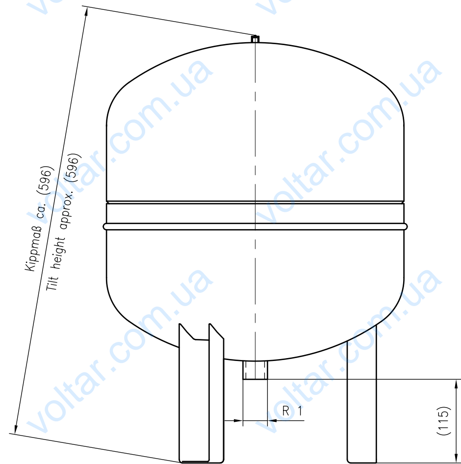
Side view
