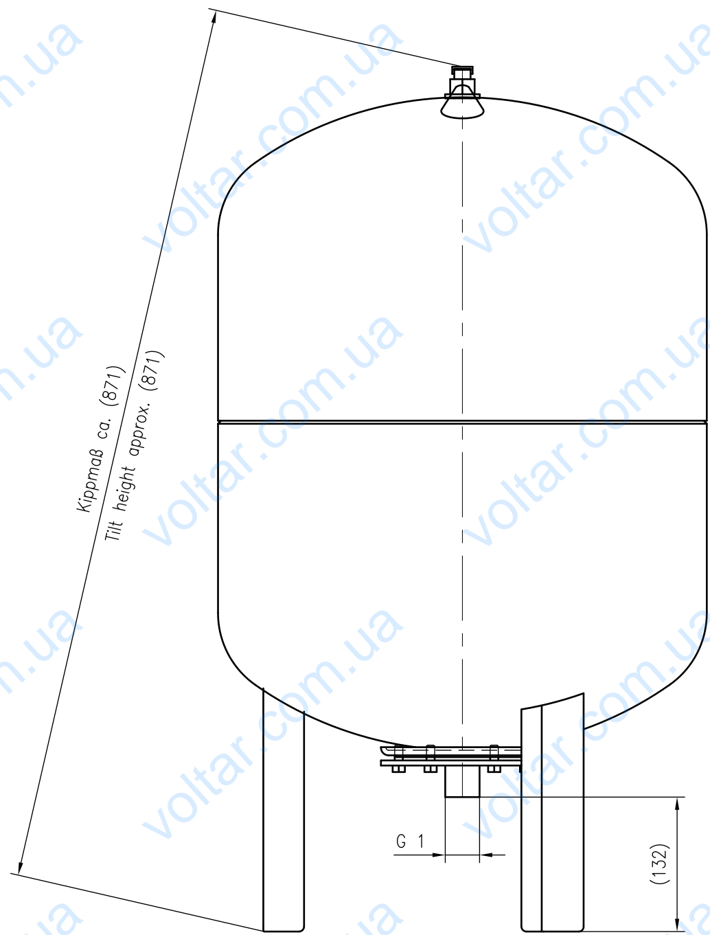
Side view
