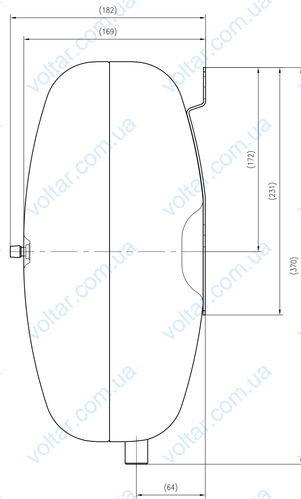
Side view
