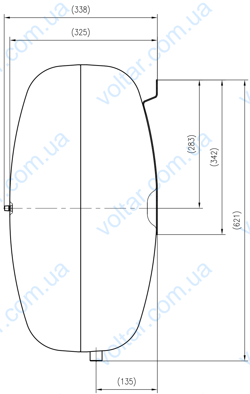
Side view
