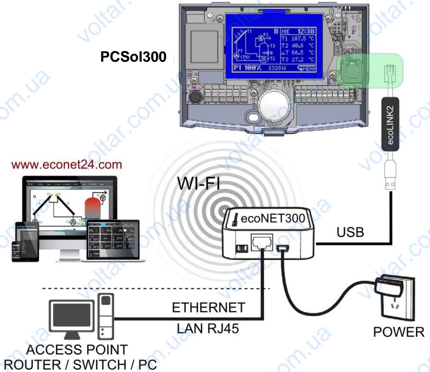
Fig. 17.12 Internet connection structure
