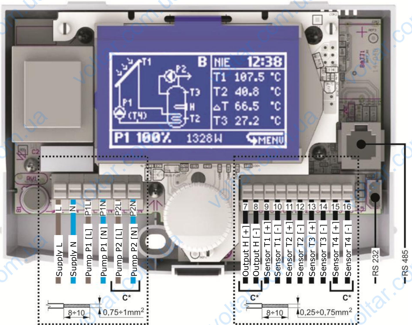
Fig. 17.3 Controller inside view with terminals
