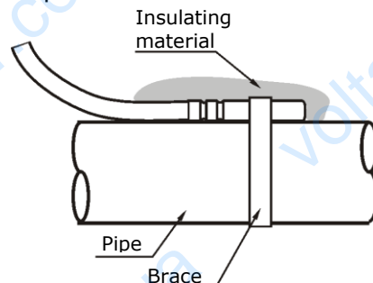
Fig. 17.9 Sensor installation on pipe surface
