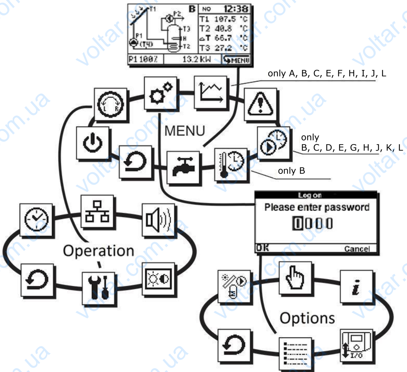
Fig. 6.5 Controller's menu structure
