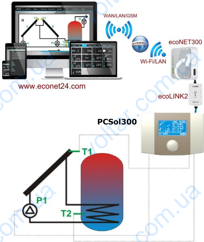
Fig. 2.1 Basic functional diagram
